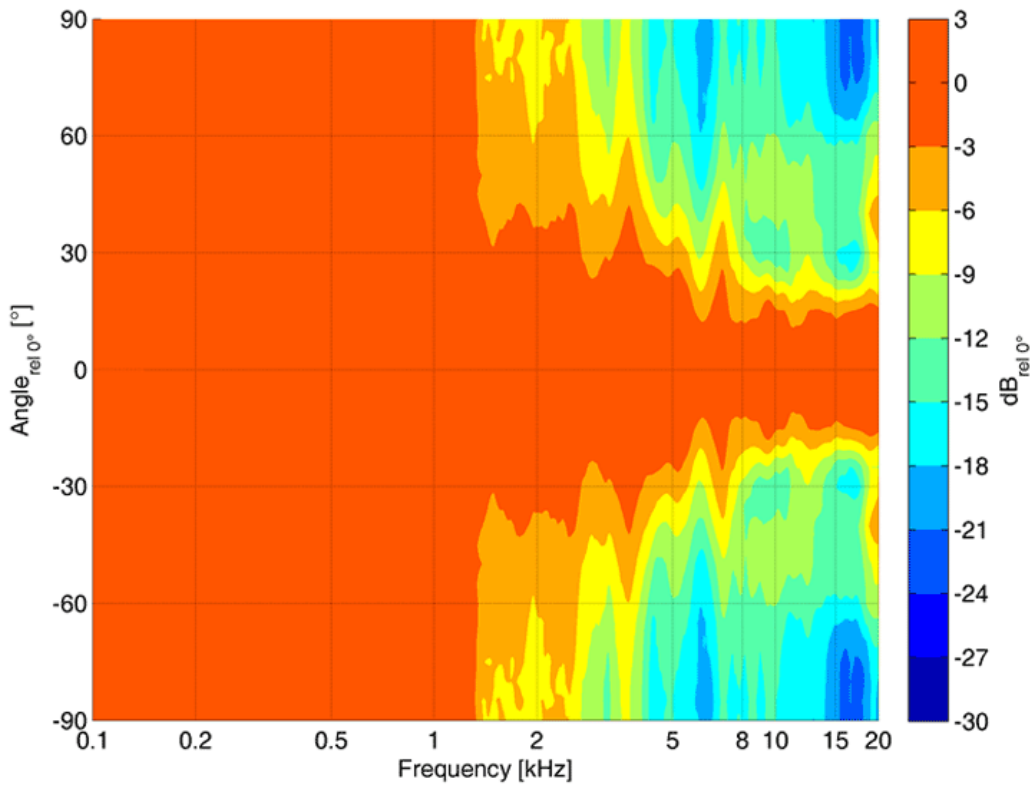
Horizontal Isobars
